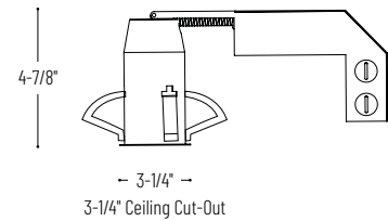
NHRIOIC-28LE4 2" Iolite IC Air-Tight Remodel Housing
